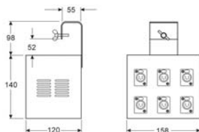
IDA6H Bar hanging type
